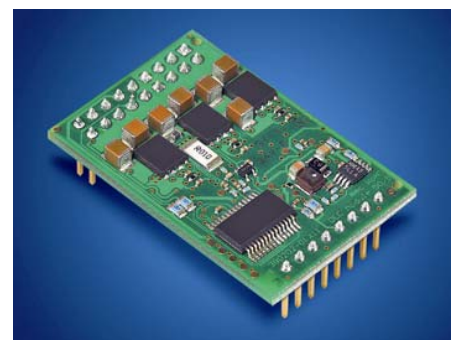
DEC module 50/5: compact speed controller for brushless DC motors with Hall sensors of up to 250 watts constant power.
